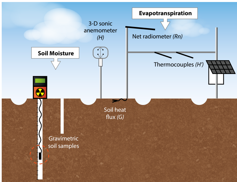
FIG. 1. Schematic of data collection on winter cover cropped and control (bare ground) fields. Illustration: Larken Root.
