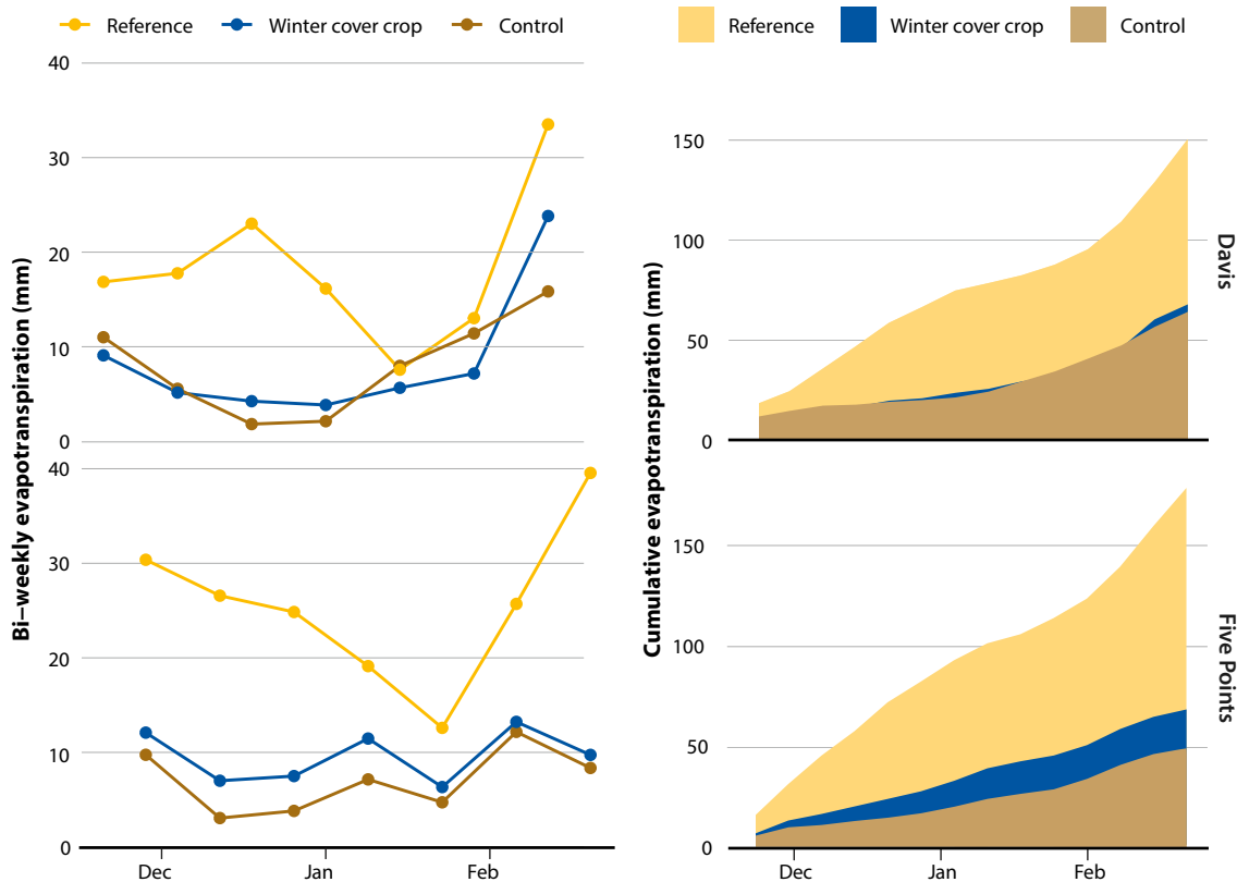
FIG. 6. Bi-weekly and cumulative actual evapotranspiration ( ET_a ) for winter cover cropped and control (bare ground) plots on annual rotation fields and reference evapotranspiration ( ET_0 ). Data was collected during the winter cover crop season of November 2017 to February 2018.
