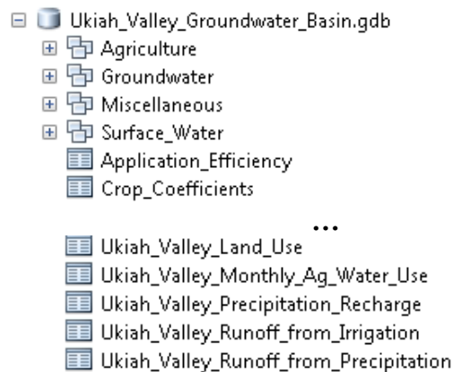
Figure 1. Geodatabase structure.
